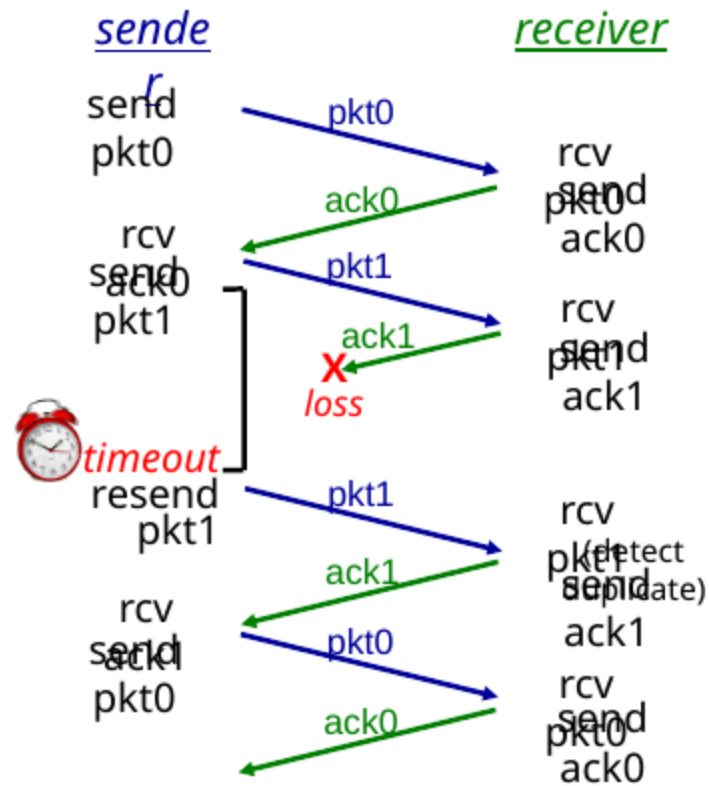
(c) ACK loss
